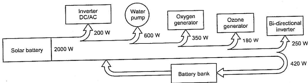
Fig. 9 Electric energy consumption in the system
