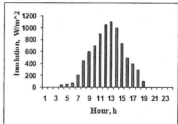
Fig. 2 The chart (day and night) insolation in Lublin between 1-3 June 2002, [3]
