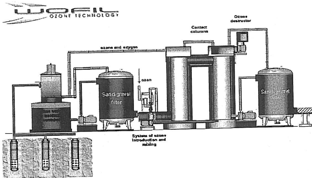
Fig. 8 WOFIL water ozonation system
