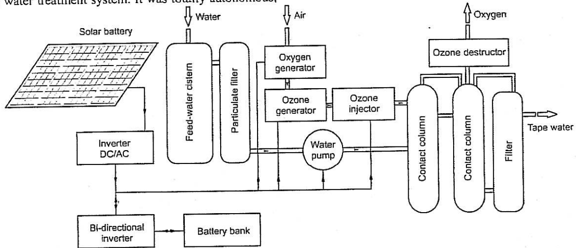
Fig. 7 Water ozonation system
